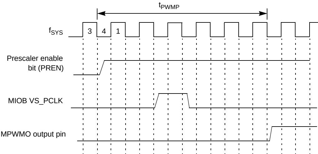
Figure F-47. MCPWM Enable to MPWMO Output Pin Rising Edge Timing Diagram
