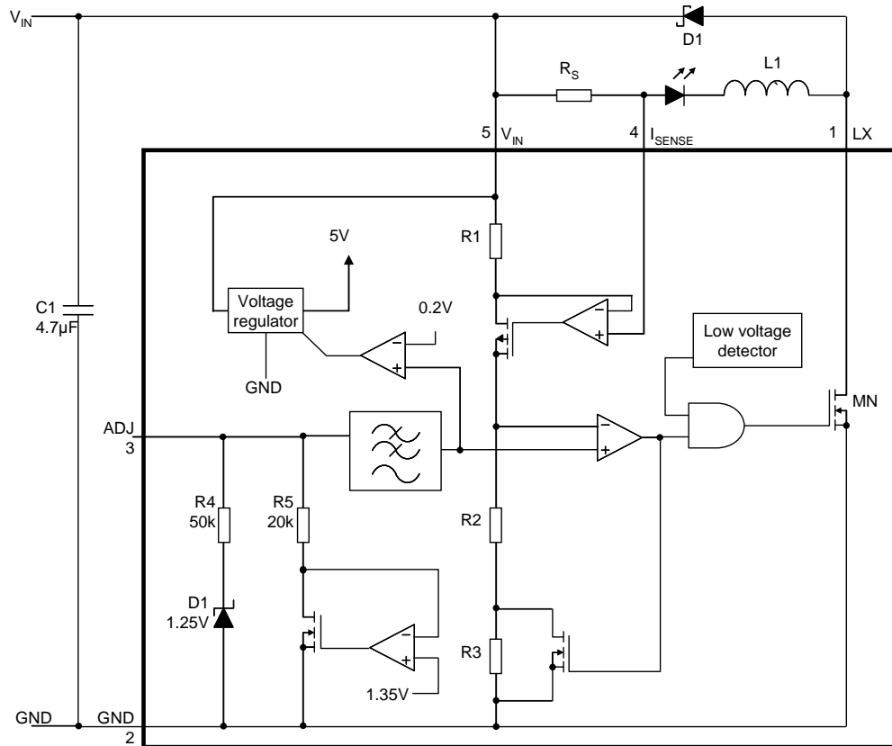
Figure 1. Block Diagram
