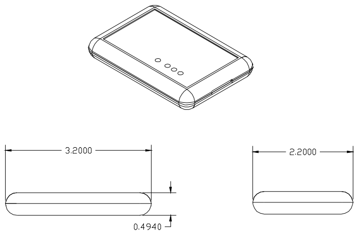
Figure 2-5. Pod Box Dimensions (in inches)
