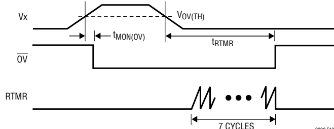
Overvoltage Timing
