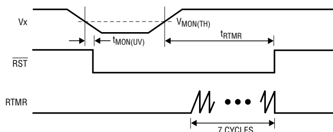
Undervoltage Timing
