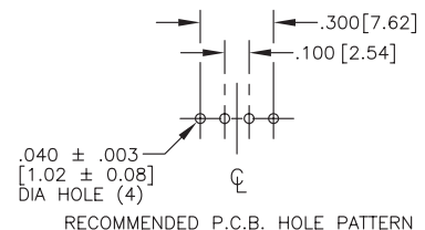
RECOMMENDED P.C.B. HOLE PATTERN
