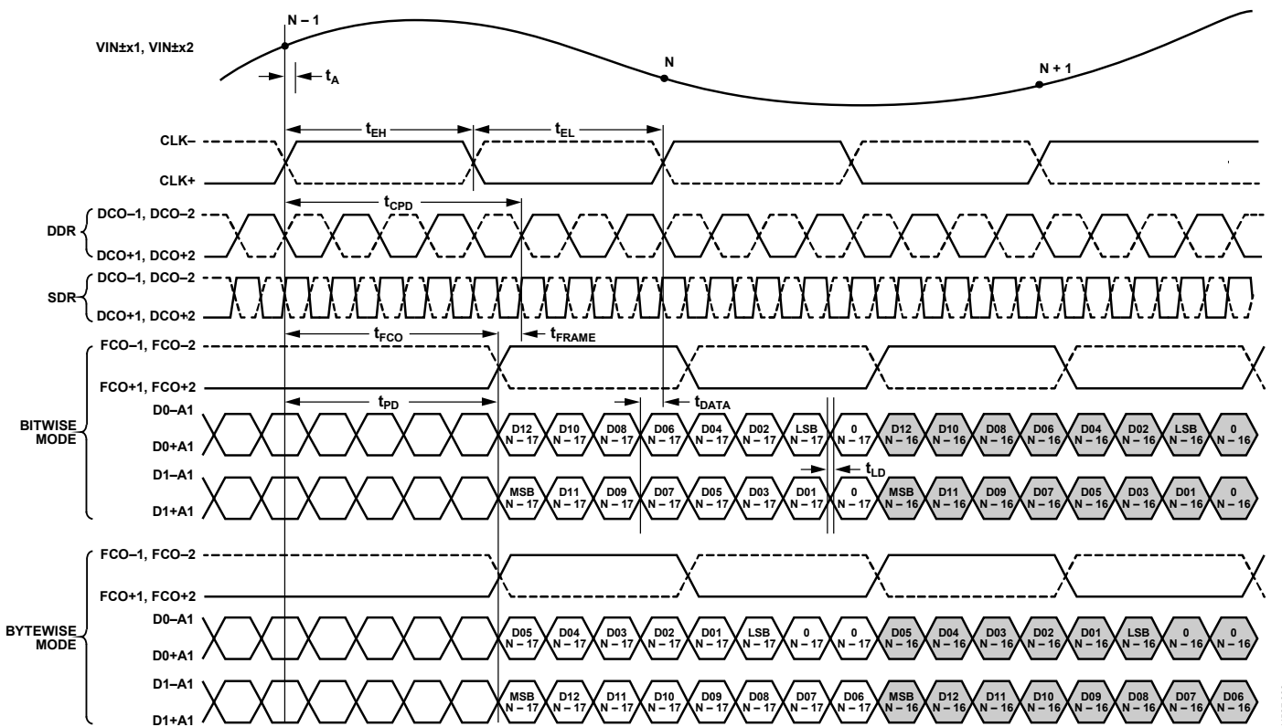
Figure 3. 16-Bit DDR/SDR, Two-Lane, 1× Frame Mode (Default)
