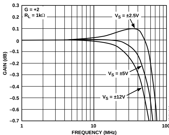
Figure 15. AD8130 Fine Scale Response vs. Supply, G = +2 , R_L = 1\ k\ \Omega
