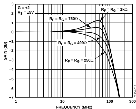
Figure 14. AD8130 Frequency Response for Various R_F/R_G
