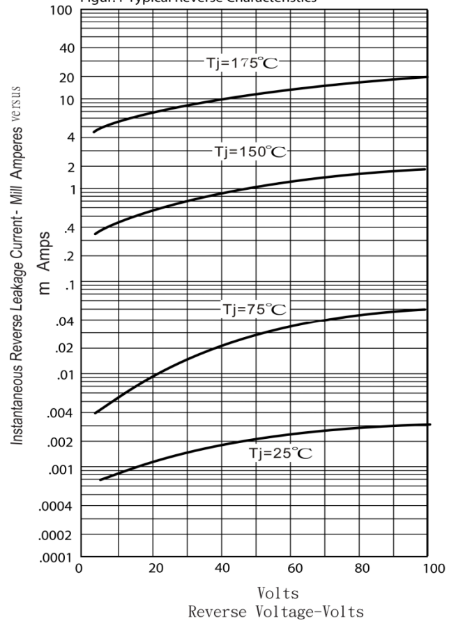
Figure.4-Typical Reverse Characteristics
