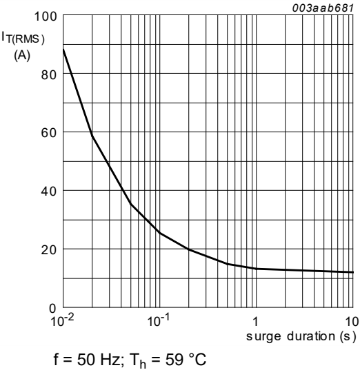
Fig. 2. RMS on-state current as a function of surge duration; maximum values f = 50 Hz; T h = 59 °C
