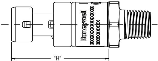
Figure 5. Electrical Connector Type Dimensions (continued)
