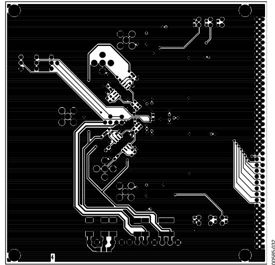
Figure 32. Bottom Routing
