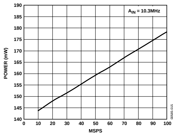
Figure 15. Analog Power Dissipation vs. Encode Rate
