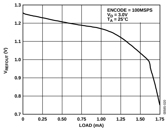
Figure 20. Voltage Reference Out vs. Current Load
