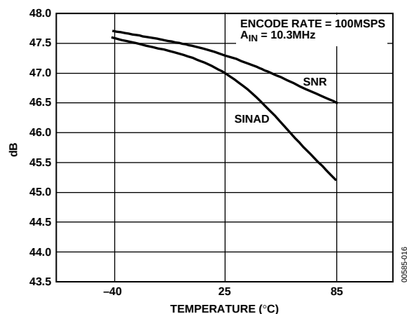
Figure 16. SINAD/SNR vs. Temperature
