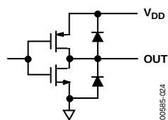
Figure 24. Equivalent Digital Output Circuit
