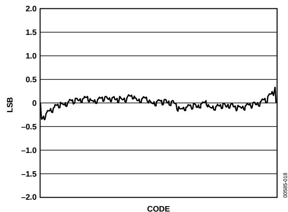
Figure 18. Integral Nonlinearity
