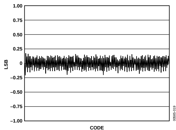
Figure 19. Differential Nonlinearity
