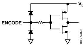
Figure 23. Equivalent Encode Input Circuit
