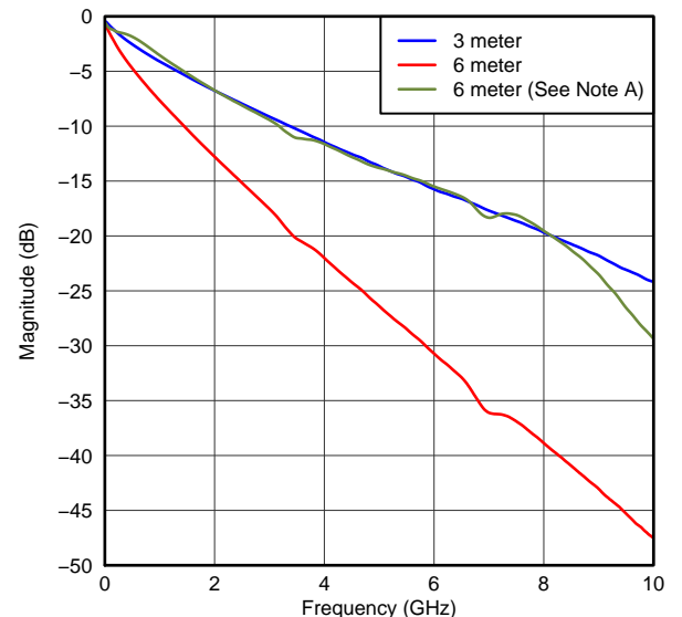
Figure 22. Trace Mode - Frequency Domain
