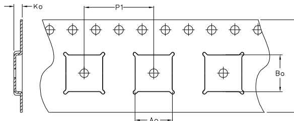
TAPE DIMENSIONS
