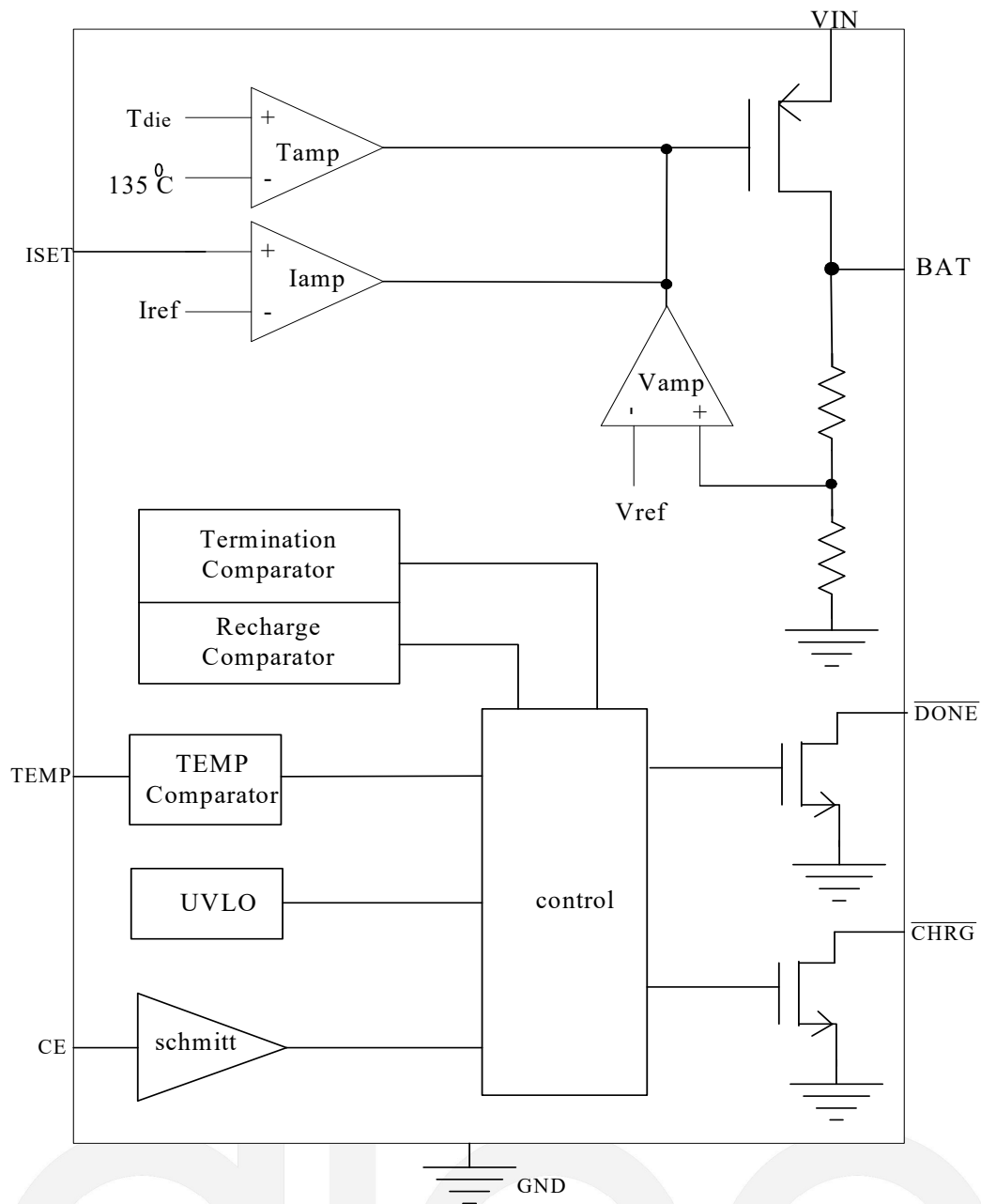
Figure 3 Block Diagram
