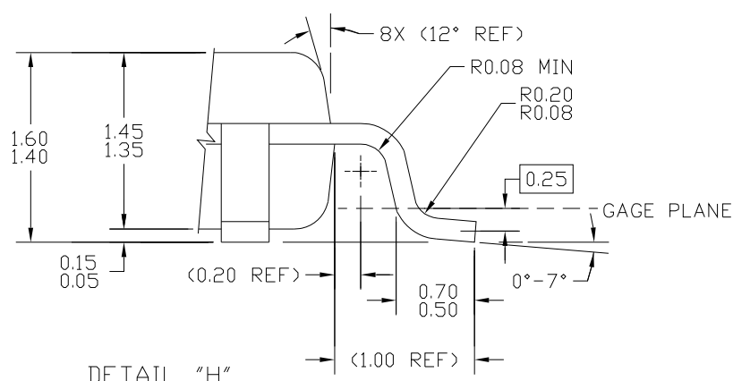
DETAIL "H"
