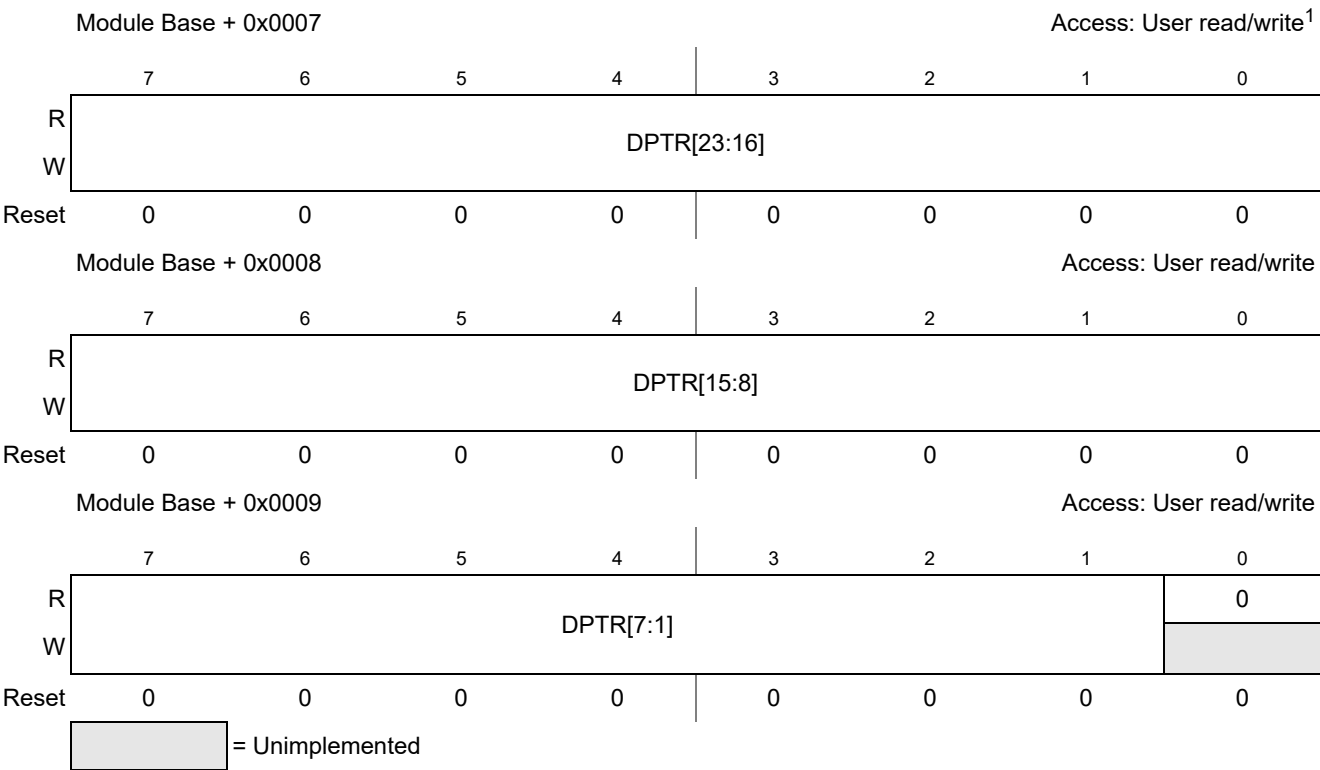
Figure 8-5. ECC Debug Pointer Register (ECDDPTRH, ECDDPTRM, ECDDPTRL)
