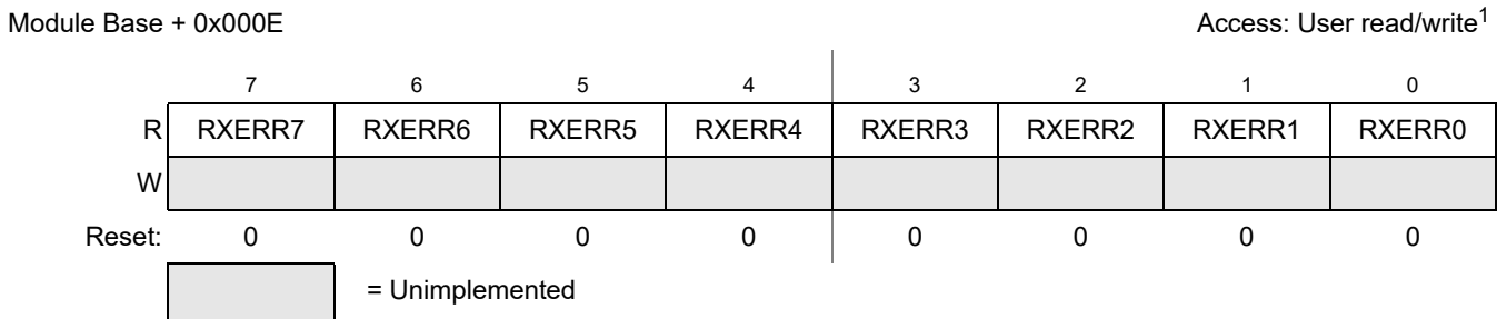
Figure 13-17. MSCAN Receive Error Counter (CANRXERR)
