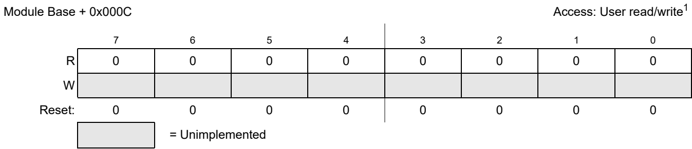
Figure 13-16. MSCAN Reserved Registers
