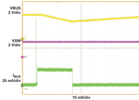
Figure 10. V_{BUS} = 5\text{ V} at 8 mA, V_{BAT} = 3.2\text{ V} , I_{in\_limit} = 100\text{ mA} , I_{CHG} = 550\text{ mA}
