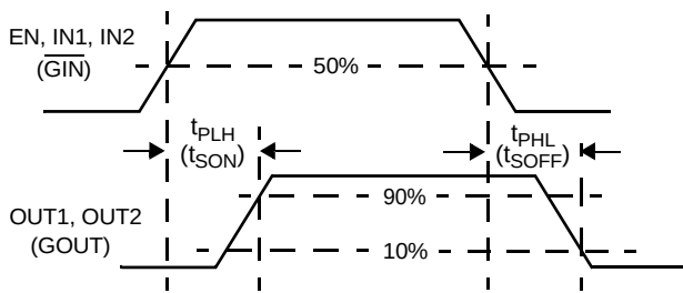
Figure 5. t_{\text{PLH}} , t_{\text{PHL}} , and t_{\text{PZH}} Timing
