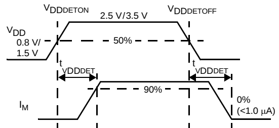
Figure 6. Low-Voltage Detection
