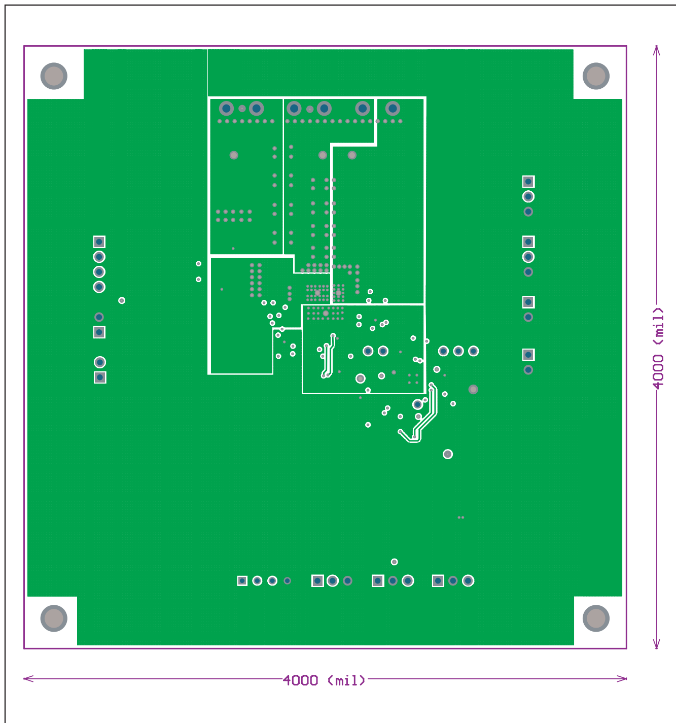
Figure 5. MAX8655 EV Kit PCB Layout—Inner Layer 2
