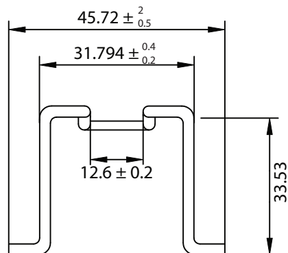
CLIP 1.80 ± 0.03mm Dia. Stainless Steel Wire
