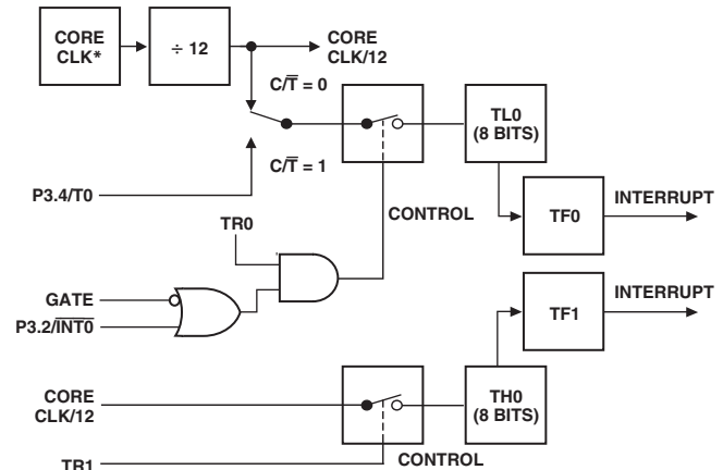
Figure 36. Timer/Counter 0, Mode 3
