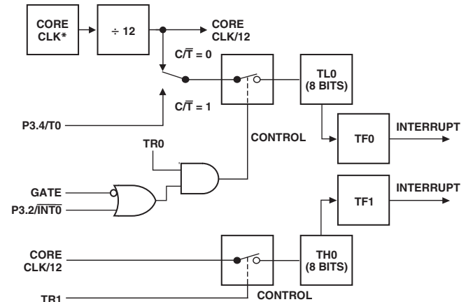
Figure 36. Timer/Counter 0, Mode 3
