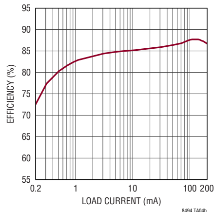
Efficiency, V_{IN} = 3.3V
