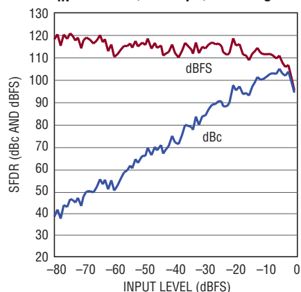
SFDR vs Input Level, f_{IN} = 70\text{MHz} , 20Mps, 2V Range
