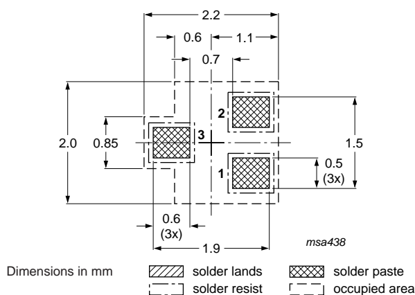
Fig 17. Reflow soldering footprint BAV70T (SOT416/SC-75)
