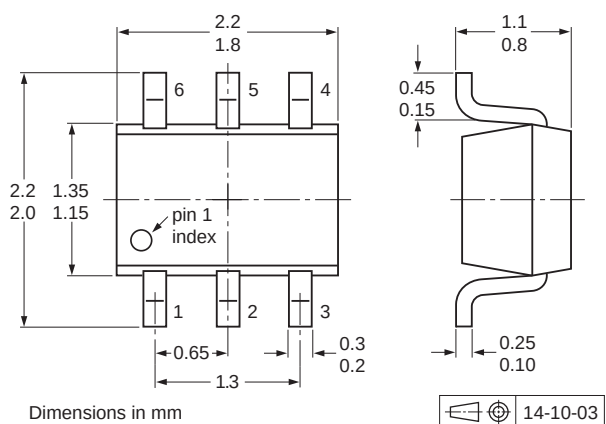
Fig 9. Package outline BAV70S (SOT363/SC-88)
