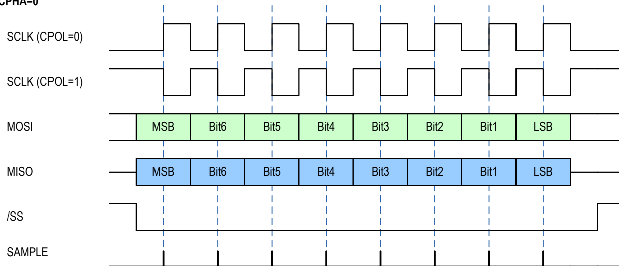
Figure 3.5 SPI Configuration CPHA=0
