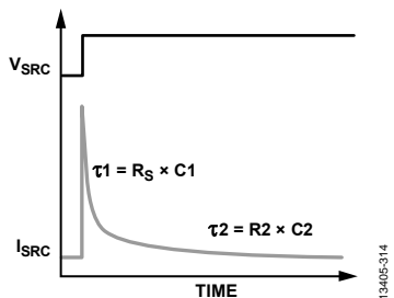
Figure 109. Step Response of Dielectric Relaxation Model
