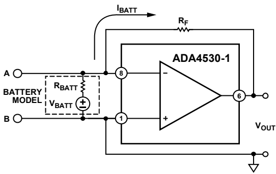
Figure 115. TIA Circuit with Contamination Battery
