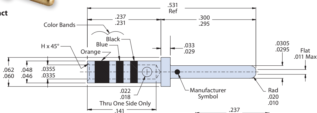
Mating End Size Wire Accomodation Military Part Number Glenair Part Number Pin 22 22-28 AWG M39029/58-360 850-002-22-360 Socket 22 22-28 AWG M39029/56-348 850-001-22-348
