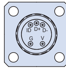
Rear Grommet View
