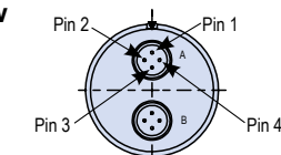
Quadrx Pin Locations
