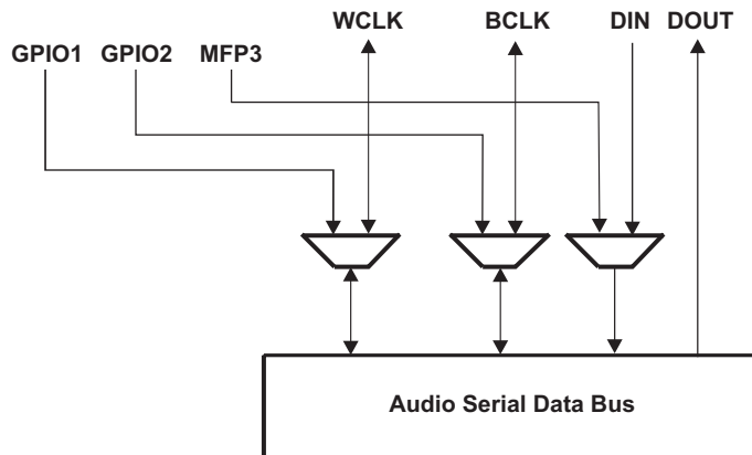
Figure 19. Alternate Audio Bus Multiplexing Function
