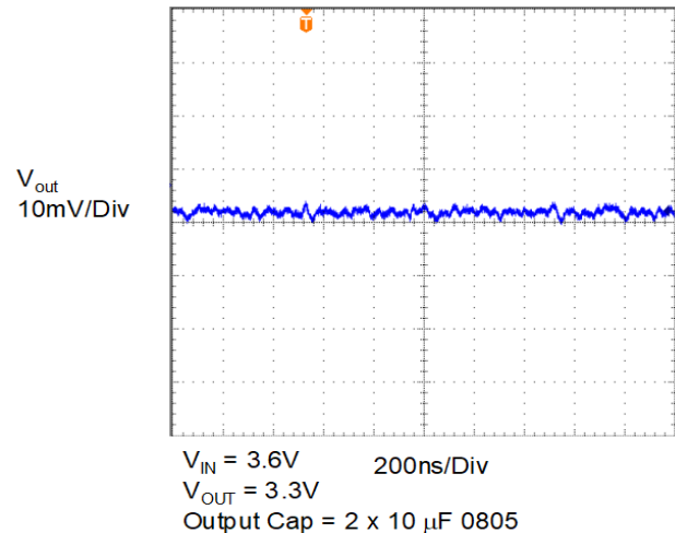
Output Ripple
