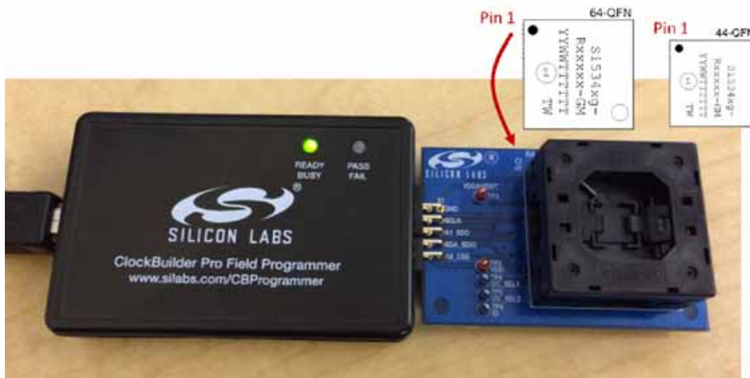
Figure 30. Correct Orientation of Device in Socket
