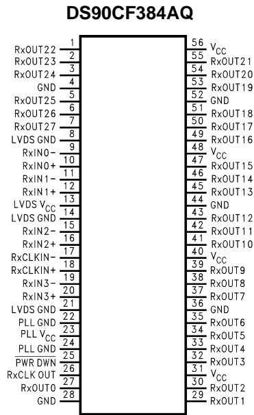
Figure 12. 56-Lead TSSOP (DGG Package)
