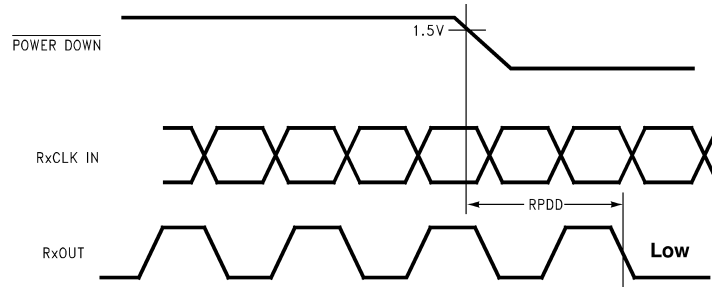
Figure 9. Receiver Power Down Delay
