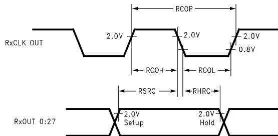
Figure 5. Receiver Output Setup/Hold and High/Low Times
