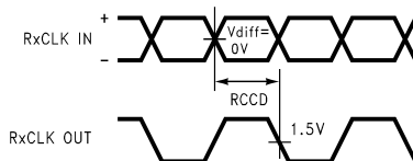
Figure 6. Receiver Clock In to Clock Out Delay
