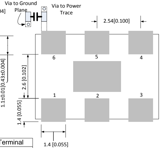
RECOMMENDED SOLDER PAD LAYOUT Units: mm [ inches]
