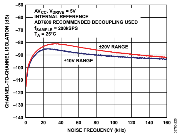
Figure 25. Channel-to-Channel Isolation
