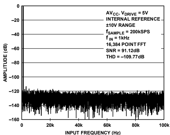
Figure 9. FFT Plot, ±10 V Range
