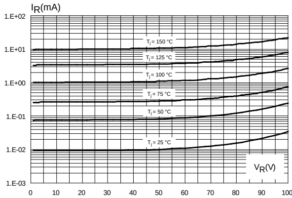
Figure 3: Reverse leakage current versus reverse voltage (typical values)
