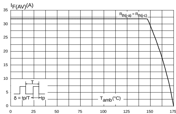
Figure 1: Average forward current versus ambient temperature ( \delta = 0.5 )
