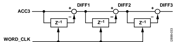
Figure 33. Differentiator
