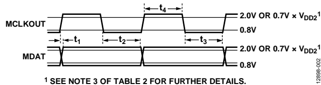
Figure 2. Data Timing
