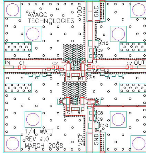
Figure 44. Demoboard
