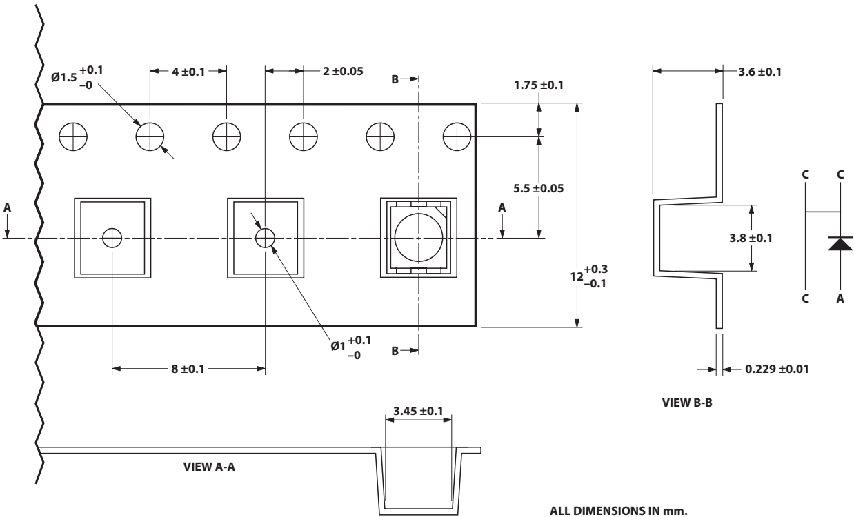
Figure 14: Tape Dimensions
