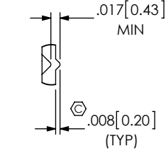
CRIMP DETAIL SCALE: 4:1 (TYP ALL CRIMPS)
