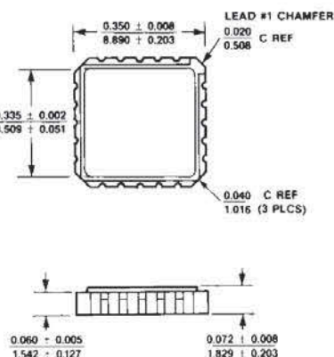
20 Leadless Chip Carrier (LP)
