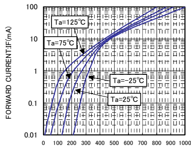
FORWARD VOLTAGE:VF(mV) VF-IF CHARACTERISTICS VF分布
