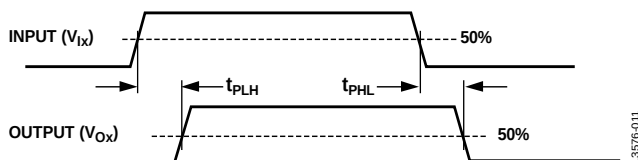
Figure 22. Propagation Delay Parameters
