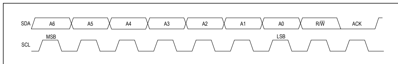
Figure 7. Slave Address
