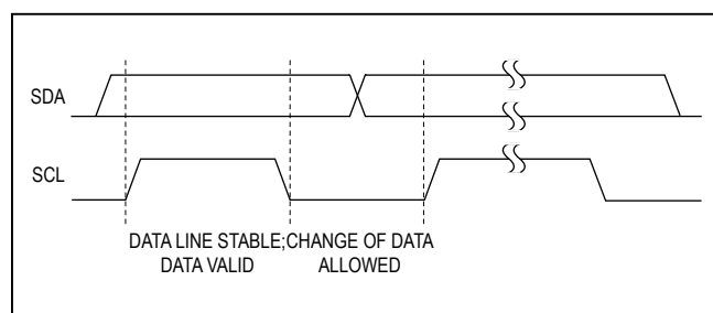
Figure 5. Bit Transfer
