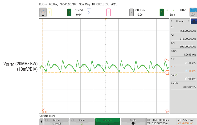
Figure 5. Output Voltage Ripple at V_{IN} = 12V , V_{OUT0} = 1V , I_{OUT0} = 30A
