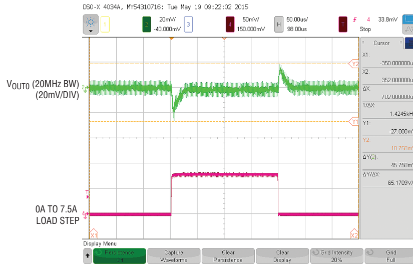
Figure 6. Transient Response at V_{IN} = 12V , V_{OUT0} = 1V , \Delta I_{OUT0} = 7.5A
