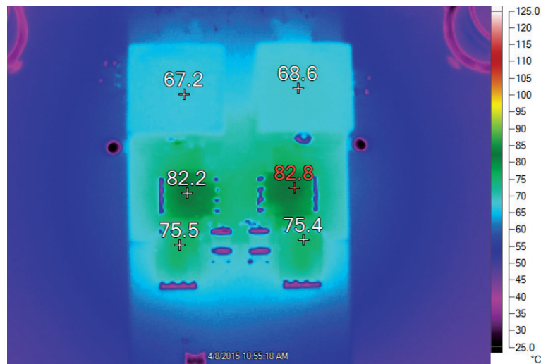
Figure 7. Thermal Performance at V_{IN} = 12V , V_{OUT0} = 1.0V , I_{OUT0} = 30A , V_{OUT1} = 1.0V , I_{OUT1} = 30A , T_A = 23.6^\circ C , No Airflow
